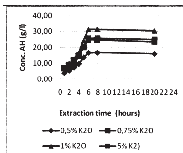
Fig. 2. Evolution of the amount of humic acid extracted depending on the alkali concentration ( \text{KOH} ), respectively 0.5% \text{K}_2\text{O} (1); 0.75% \text{K}_2\text{O} (2); 1% \text{K}_2\text{O} (3); 5% \text{K}_2\text{O} (4) and 10% \text{K}_2\text{O} (5) and different times
