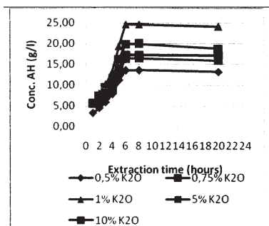
Fig. 1. Evolution of the amount of humic acid extracted depending on the alkali concentration ( \text{K}_2\text{CO}_3 ), respectively 0.5% \text{K}_2\text{O} (1); 0.75% \text{K}_2\text{O} (2); 1% \text{K}_2\text{O} (3); 5% \text{K}_2\text{O} (4) and 10% \text{K}_2\text{O} (5) and different times
