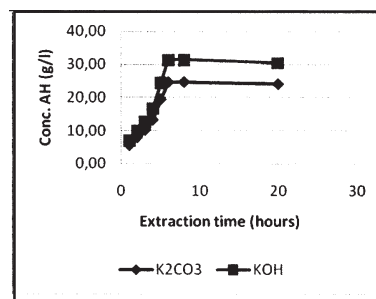
Fig. 4 Evolution of the amount of humic acids extracted depending on the nature of the alkali ( K_2CO_3 respectively KOH) for a concentration of 1% K_2O and different times
